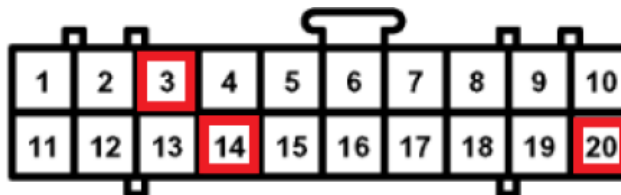
Wire side of vehicle's Blue radio connector
